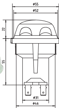
MG1448 (Max.25W; Pin: 90° & 180° available)
